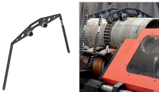
DCS-0436-12-00-00-0 Clamping device for short pipes of 400-830 mm length
