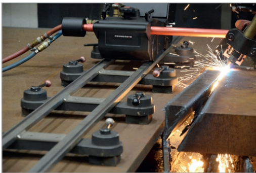
Standard Torch Holder 28-35 mm (1.10"-1.38") ZCS-0475-28-10-00-0
